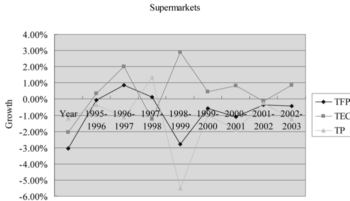
Figure 2B. TFP, TEC and TP Dynamics of Supermarkets
