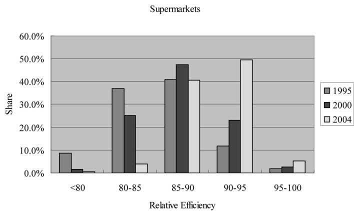
Figure 3B. Distribution of Efficiency Scores for Supermarkets
