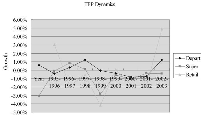
Figure 1. TFP Dynamics and Demand Fluctuation
