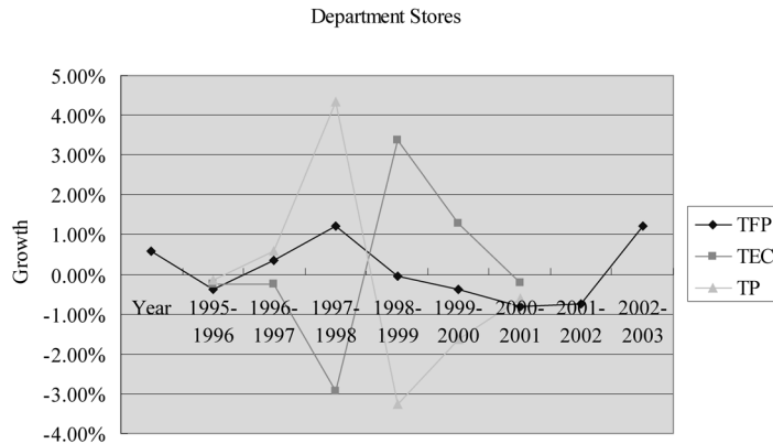
Figure 2A. TFP, TEC and TP Dynamics of Department Stores
