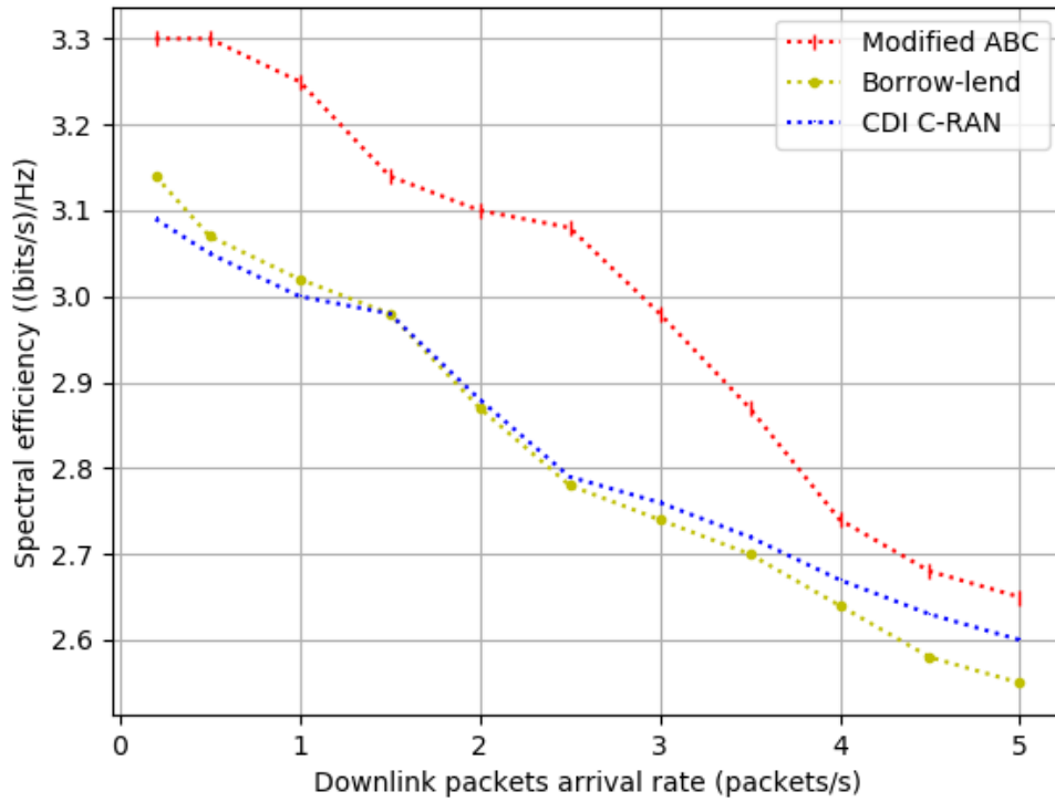
Figure 13 Spectral efficiency
